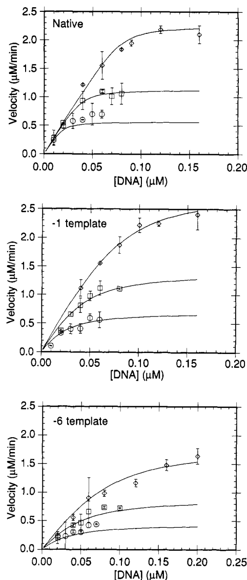
FIGURE 2: Comparison of representative steady-state kinetic fits for initiation of transcription from the native promoter ( K_m = 2.0 nM; k_{\text{cat}} = 28.3 min ^{-1} ), the promoter containing dU at position -1 on the template strand ( K_m = 12.5 nM; k_{\text{cat}} = 35.2 min ^{-1} ), and the promoter containing dU at position -6 on the template strand ( K_m = 23 nM; k_{\text{cat}} = 22.6 min ^{-1} ). The enzyme concentrations are (○) 0.02, (□) 0.04, and (◇) 0.08 \mu\text{M} . Other details of the experiment are described in the text.
